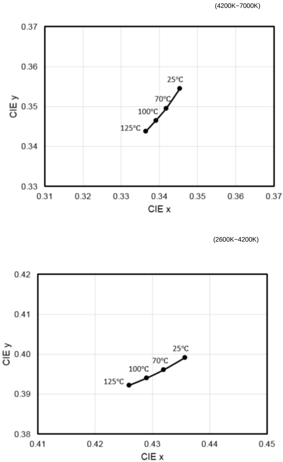
Fig 8. Chromaticity Coordinate vs. Junction Temperature, I_F=65mA
