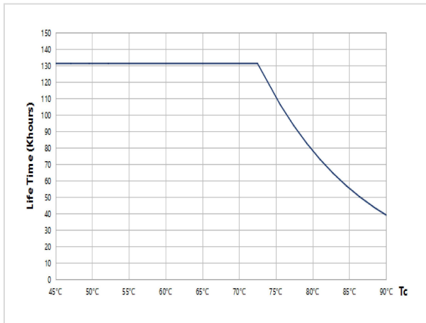
Lifetime Curve
